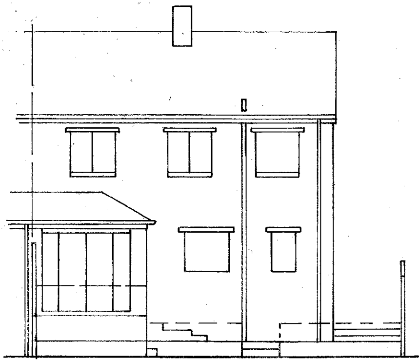
EXISTING REAR 1:100
