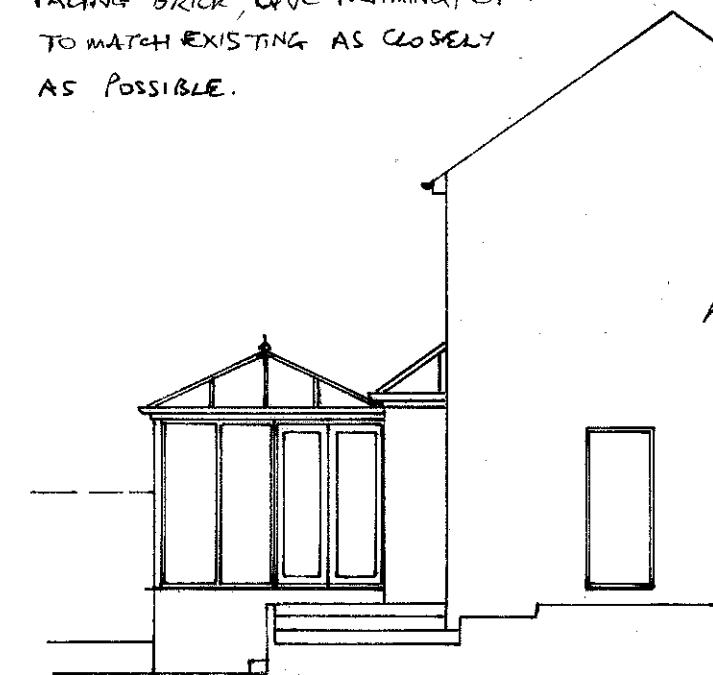
PROPOSED SIDES 1:100
